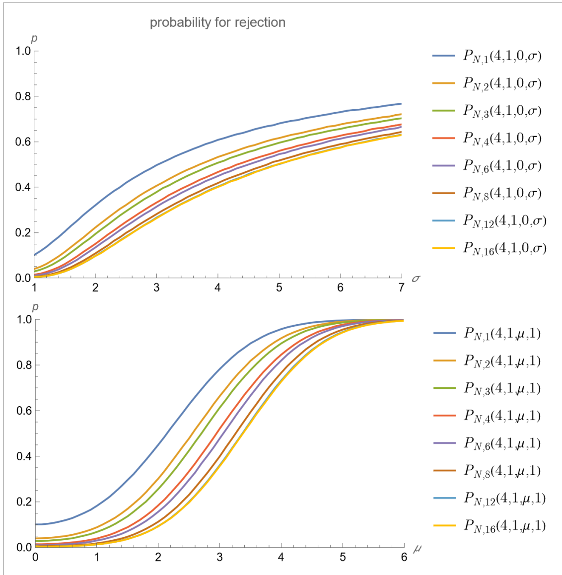
Figure 111: P_{N,a}(4,1,\mu,\sigma)
