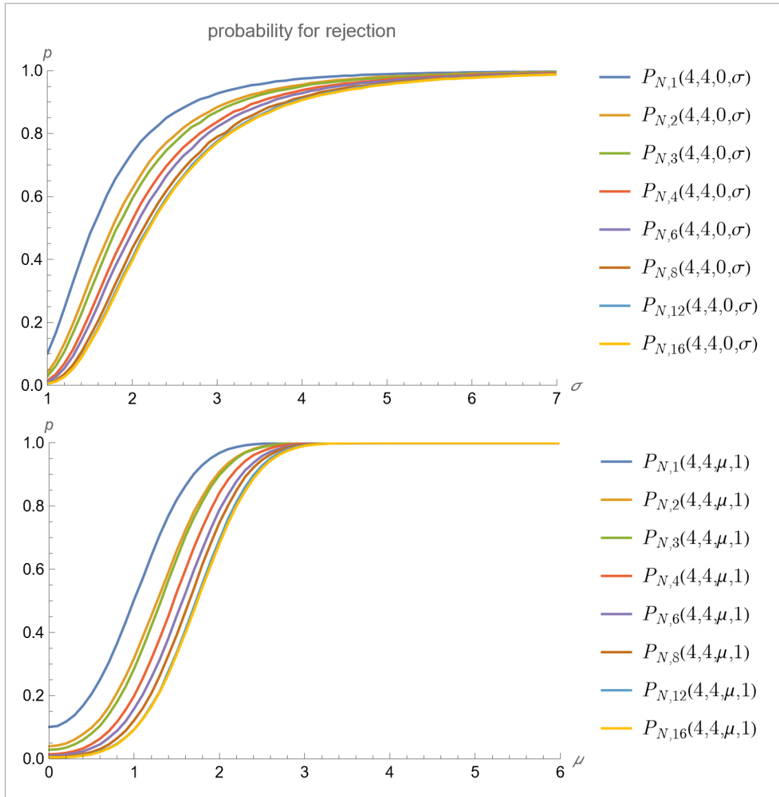
Figure 114: P_{N,a}(4,4,\mu,\sigma)
