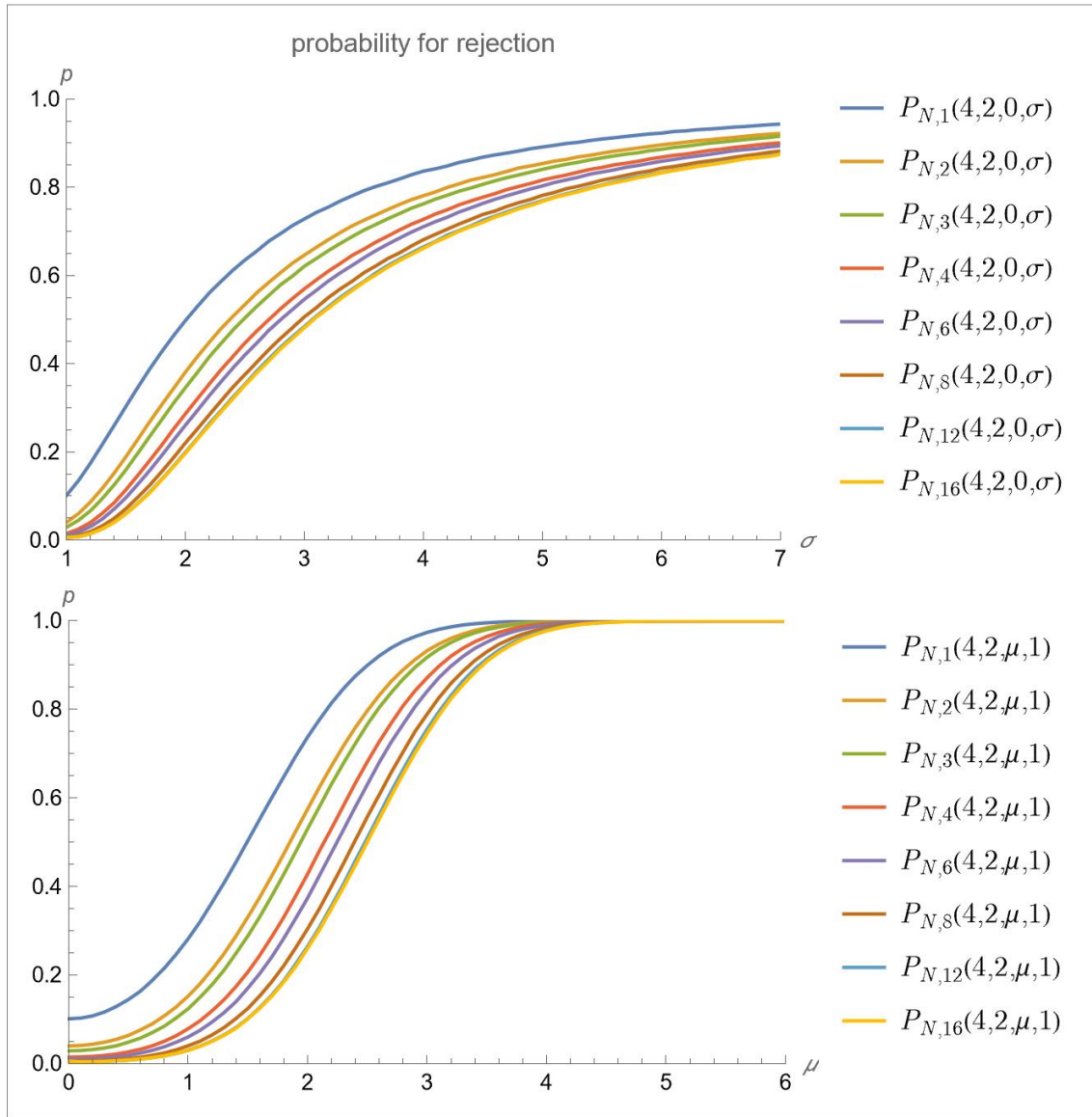
Figure 112: P_{N,a}(4,2,\mu,\sigma)
