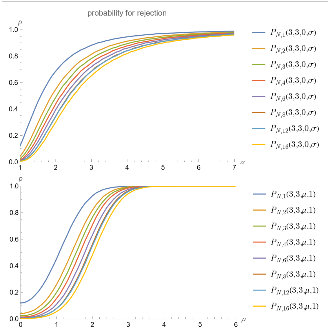
Figure 110: P_{N,a}(3,3,\mu,\sigma)
