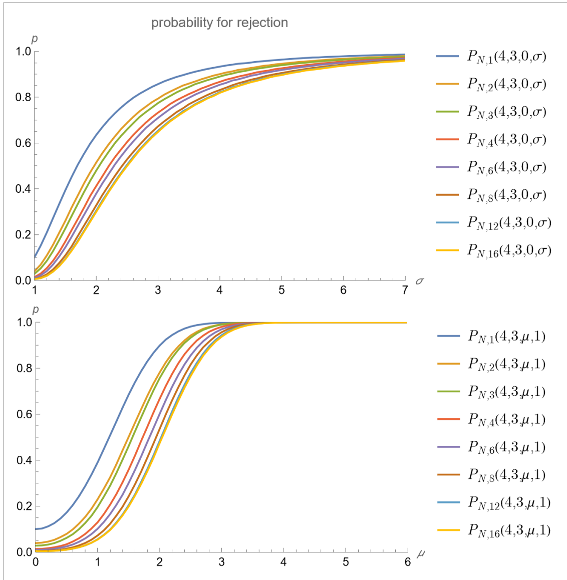
Figure 113: P_{N,a}(4,3,\mu,\sigma)
