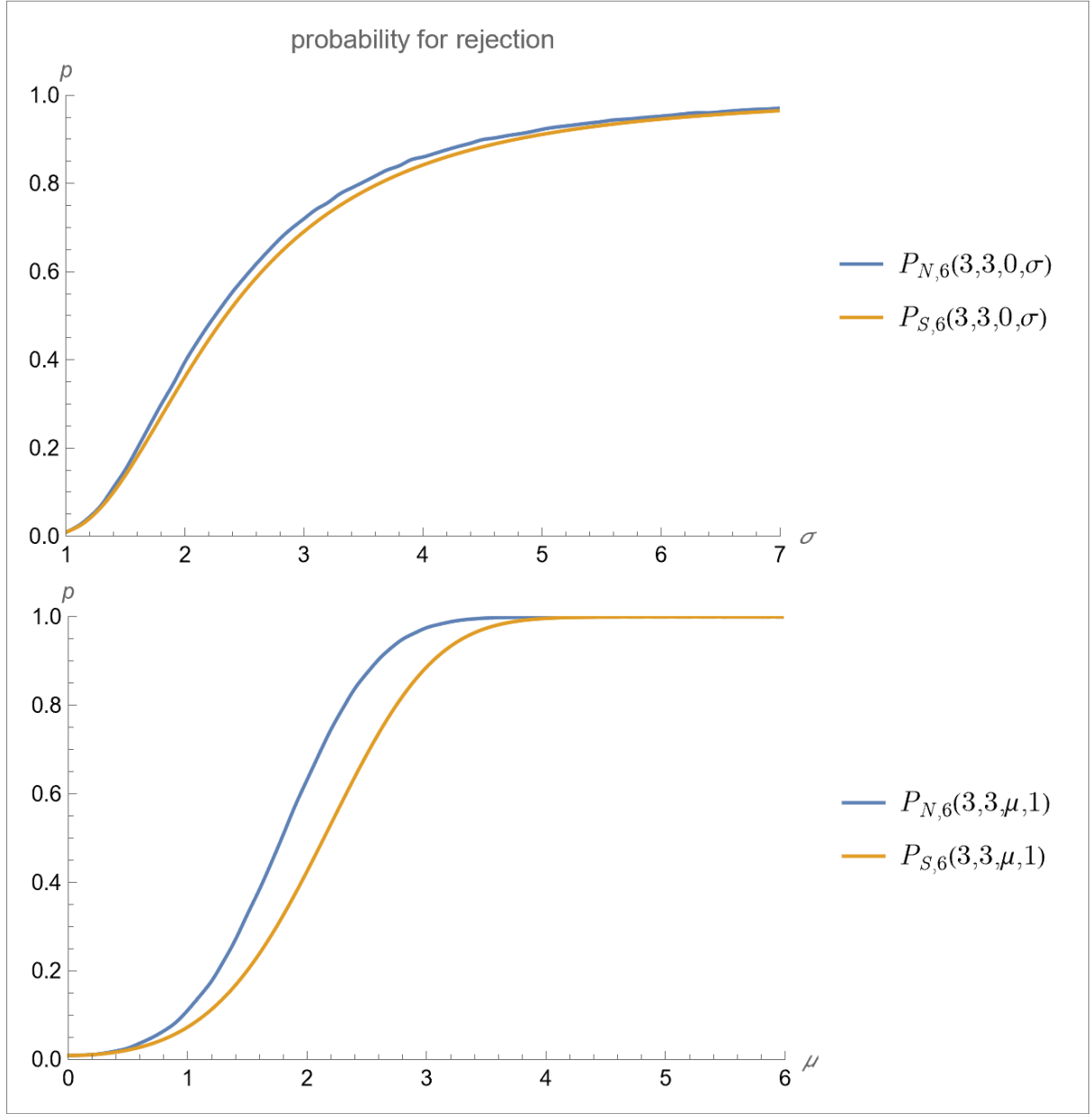
Figure 3. The probabilities for rejection of the CNN N_6(x_1, x_2, x_3) when applied to three QC measurements, distributed as \mathcal{N}(0, \sigma^2) ( upper plot ) or as \mathcal{N}(\mu, 1) ( lower plot )
