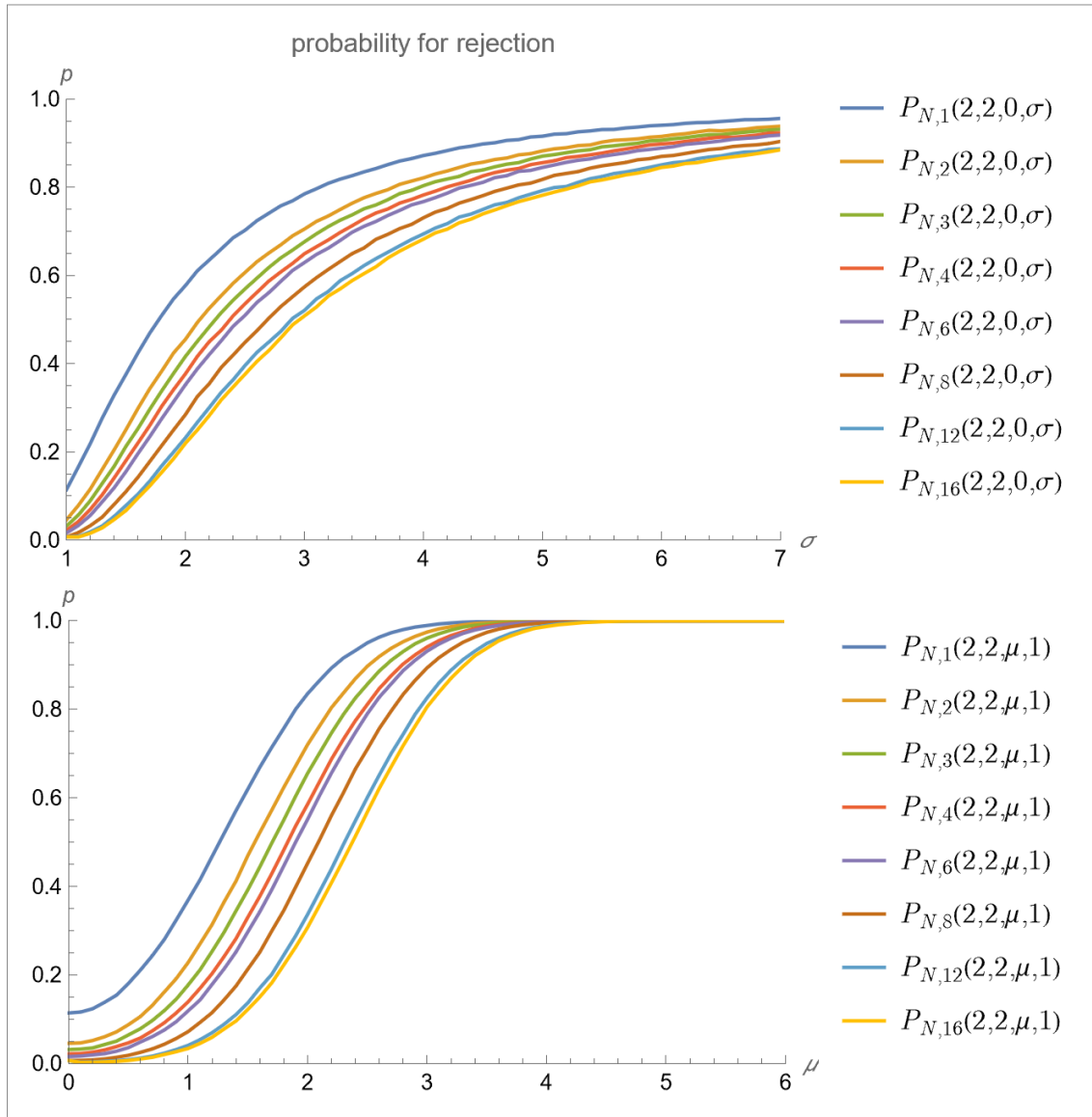
Figure 107: P_{N,a}(2,2,\mu,\sigma)
