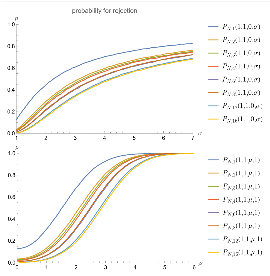
Figure 105: P_{N,\alpha}(1,1,\mu,\sigma)
