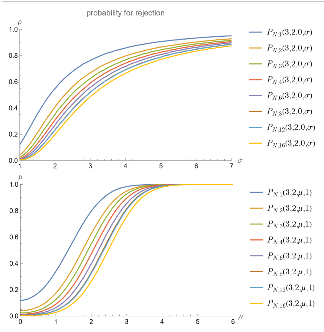
Figure 109: P_{N,a}(3,2,\mu,\sigma)
