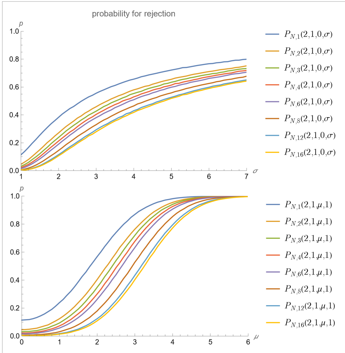
Figure 106: P_{N,\alpha}(2,1,\mu,\sigma)
